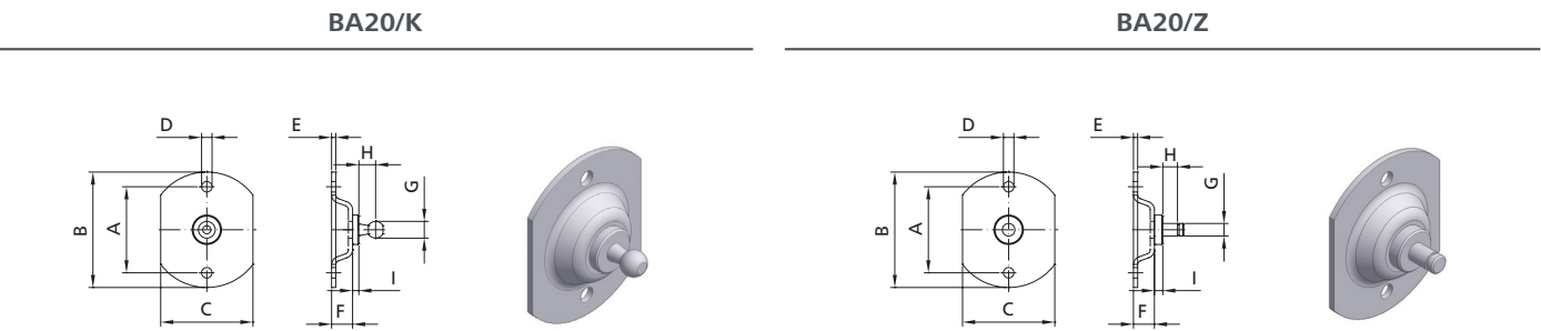
Round bracket
