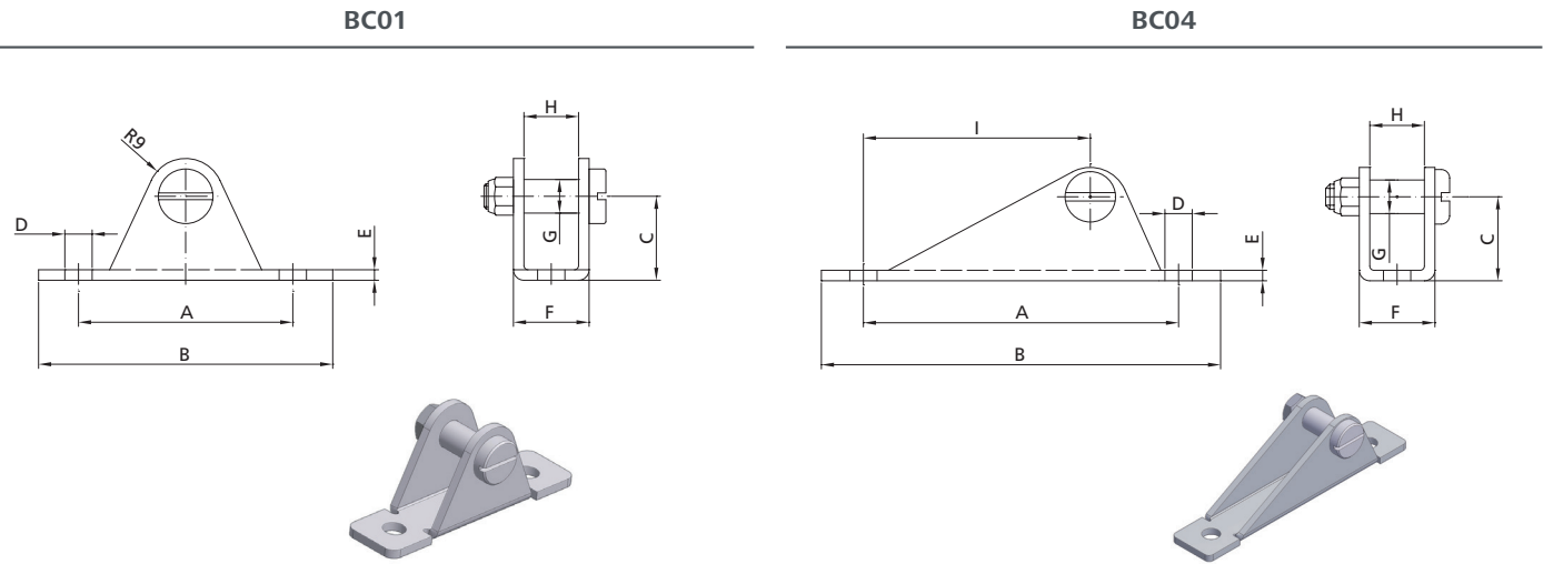
Clevis bracket
